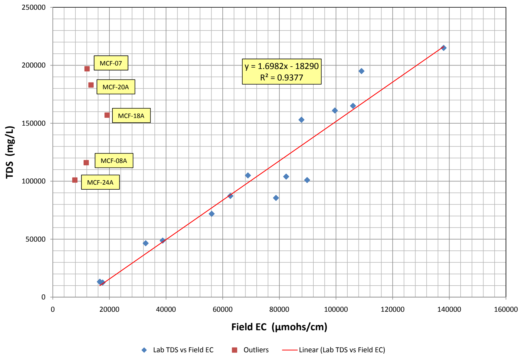
Figure 3: High Range Lab TDS vs Field EC
