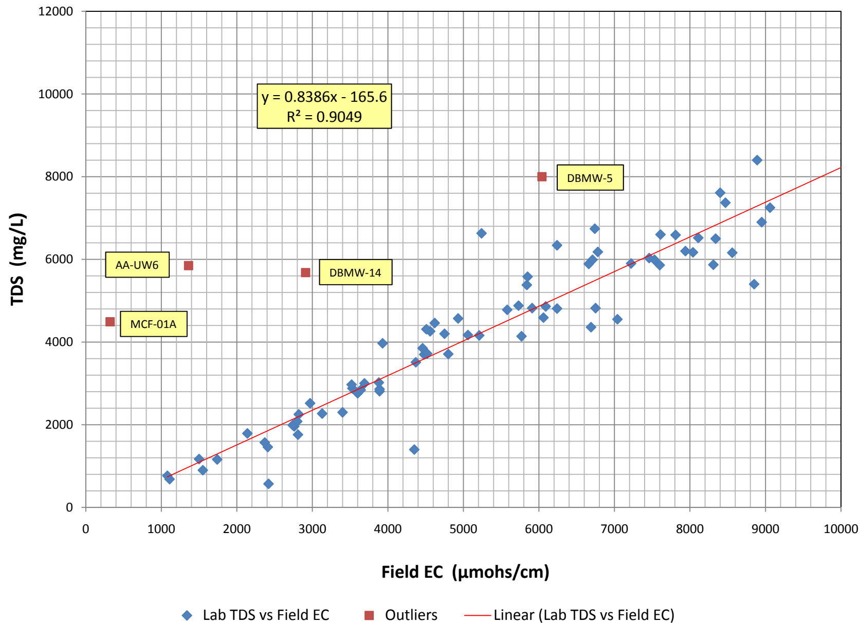
Figure 2: Low Range Lab TDS vs Field EC
