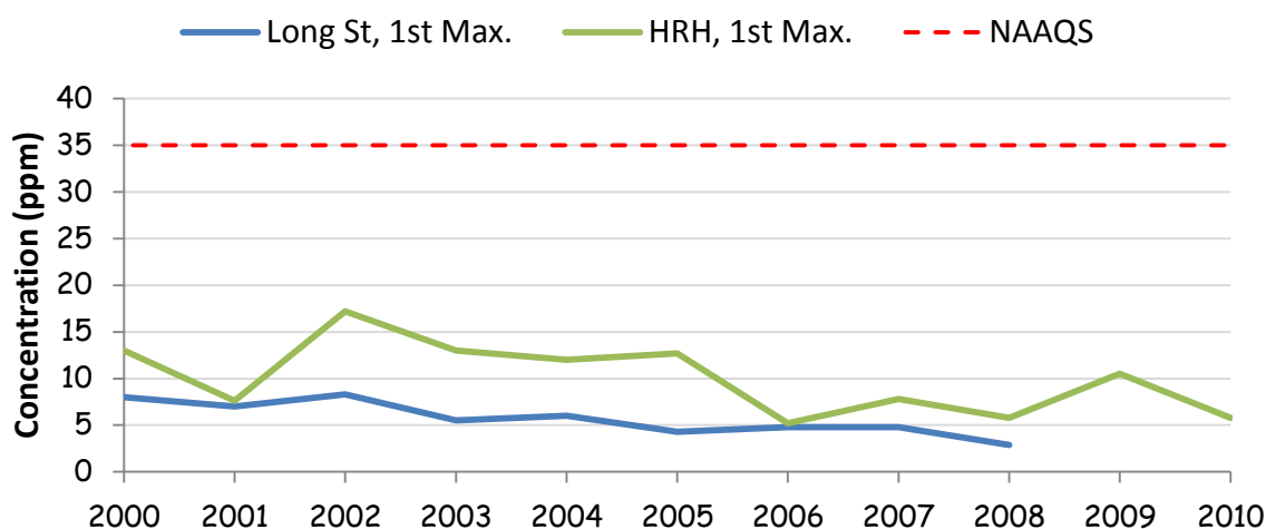
Figure 3: Carbon Monoxide (1-hour Average) for the Long St. and Harvey's Resort Hotel (HRH) monitoring stations. The 1 st highest values, are shown for both monitor sites. NAAQS (35 ppm) is shown with a red dashed line.
