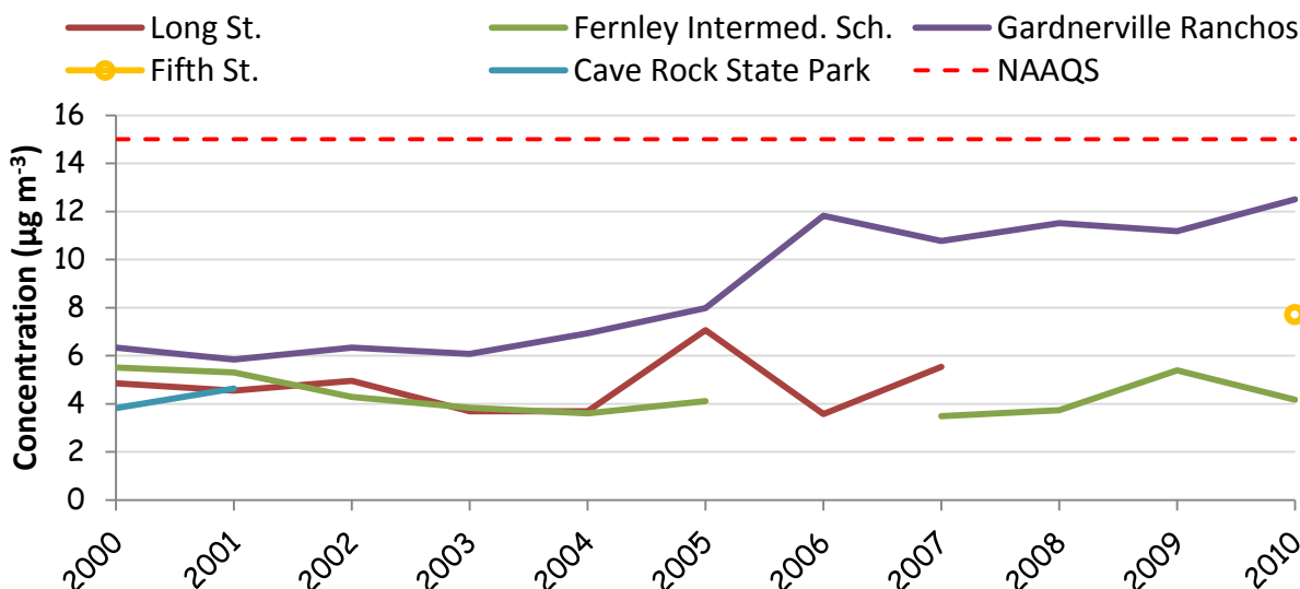
Figure 14: Annual averages of \text{PM}_{2.5} concentrations. The 1997 NAAQS ( 15 \mu\text{g}/\text{m}^3 ) is shown as well.
