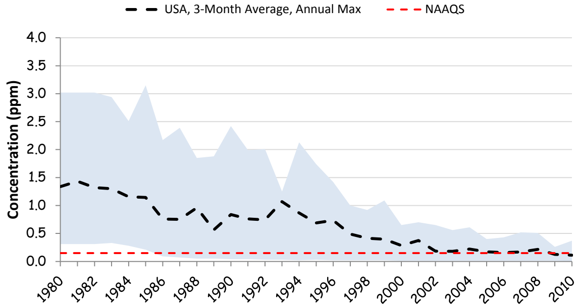
Figure 5: National lead trend, 1980-2010. The black dashed line is the annual 1 st -highest value (i.e., the annual maximum) based on 31 (1980-1989), 62 (1990-1999), and 92 (2000-2010) monitoring sites ( http://www.epa.gov/airtrends/lead.html ). The blue area delimits the 10 th and 90 th percentile of the annual observation distributions. Red dotted line is the 2008 national standard (0.15 ppm).
