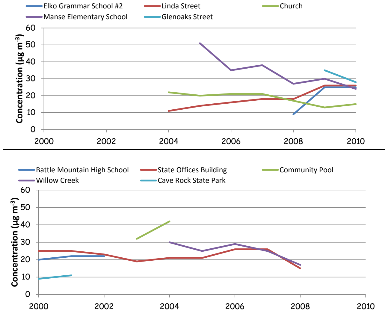
Figure 18: Annual average for PM 10 from active (above) and discontinued (below) monitors
