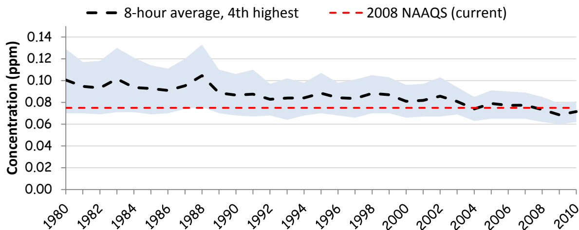
Figure 7: National ozone trend, 1980-2010. The black dashed line is the annual 4 th highest value of the 8-hour average concentration based on 247 (1980-1989), 507 (1990-1999), and 946 (2000-2010) monitoring sites ( http://www.epa.gov/airtrends/ozone.html ). The blue area delimits the 10 th and 90 th percentile of the annual observation distributions. Red dashed line is the current 8-hour national standard (0.075 ppm, accordingly to the 2008 NAAQS). From 1997 to 2008, the 8-hour NAAQS was 0.080 ppm. From 1979 to 1997, only the 1-hour NAAQS was used.
