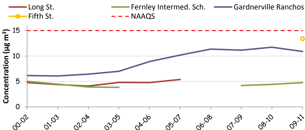
Figure 15: 3-year average of annual mean \text{PM}_{2.5} concentrations (i.e., the design values). The 1997 NAAQS ( 15 \mu\text{g}/\text{m}^3 ) is shown as well. Cave Rock State Park stations is not shown, as less than 3 consecutive years of data were available.
